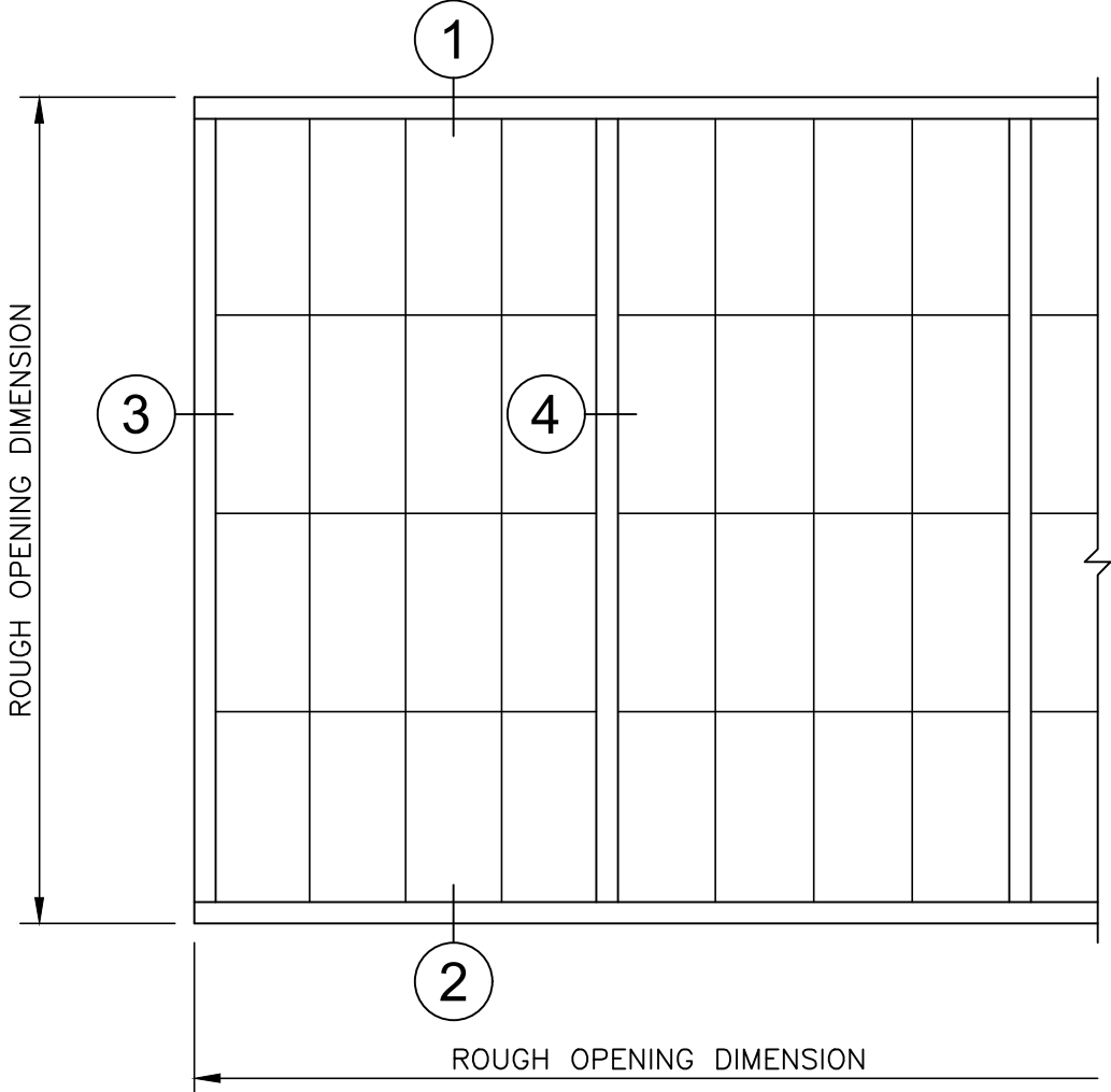
WALL ELEVATION
