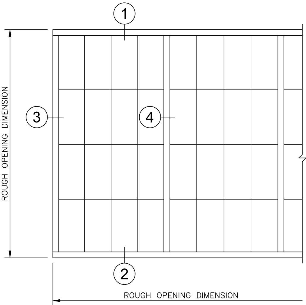
WALL ELEVATION
