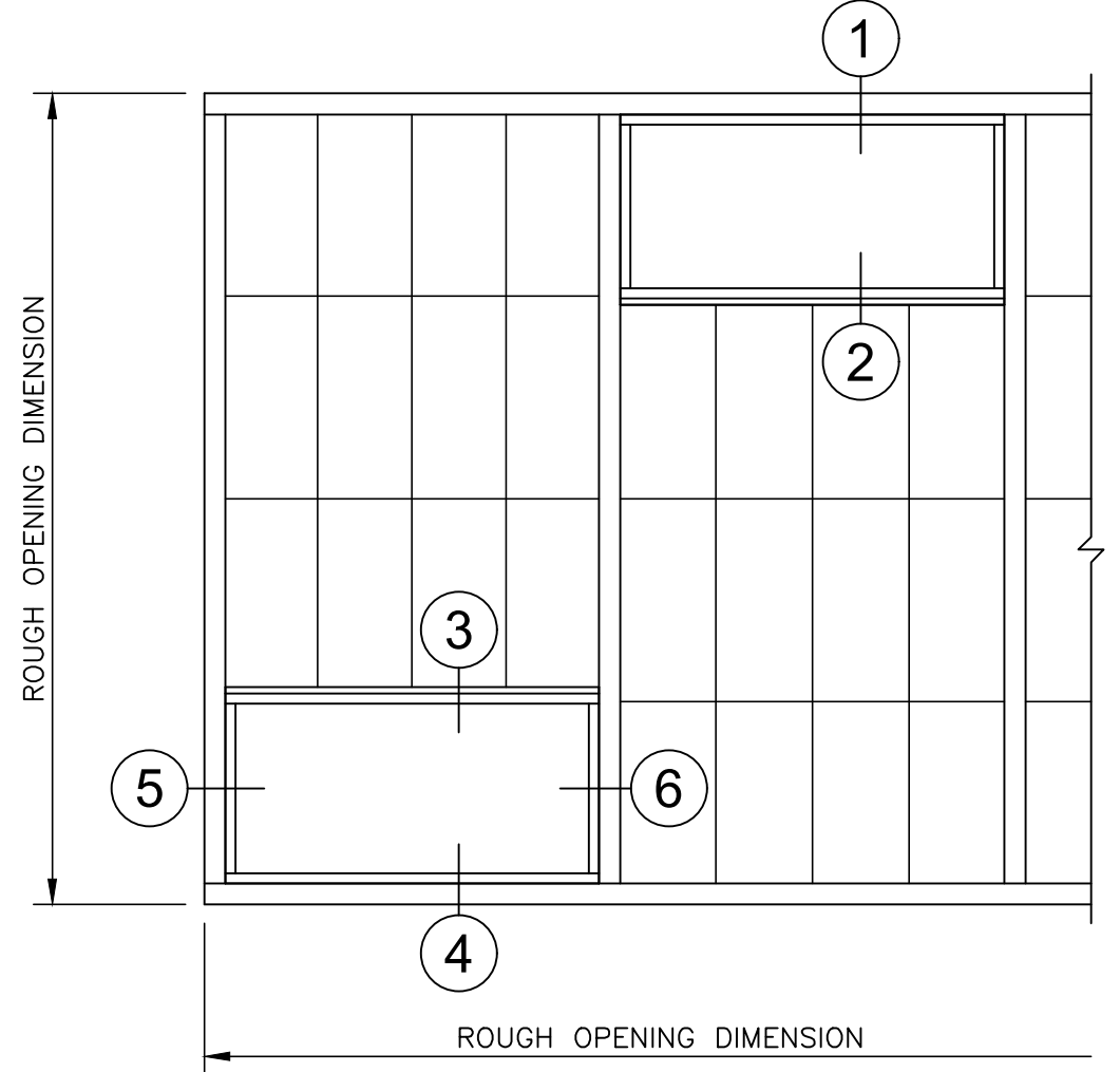
WALL ELEVATION
