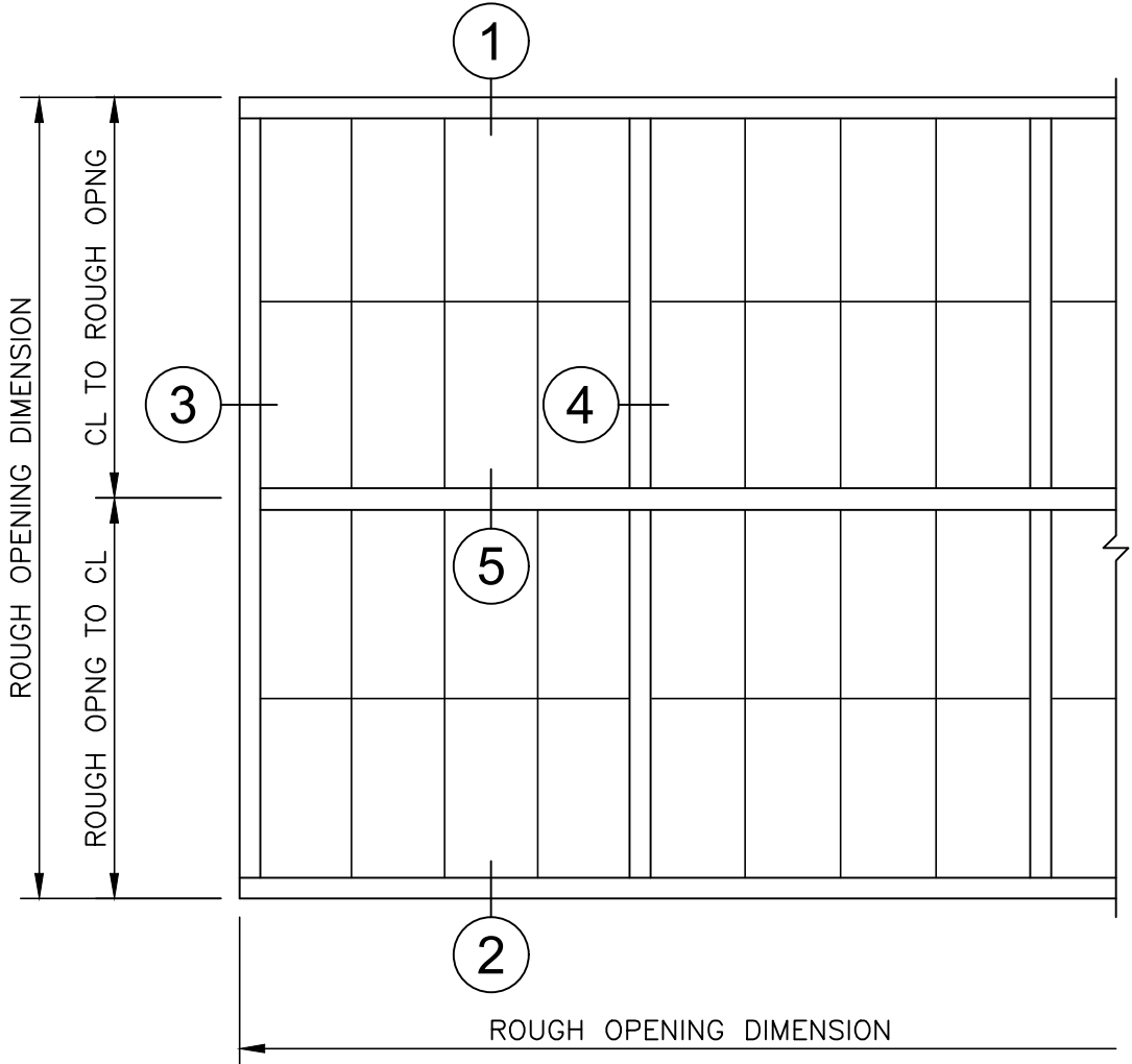
WALL ELEVATION
