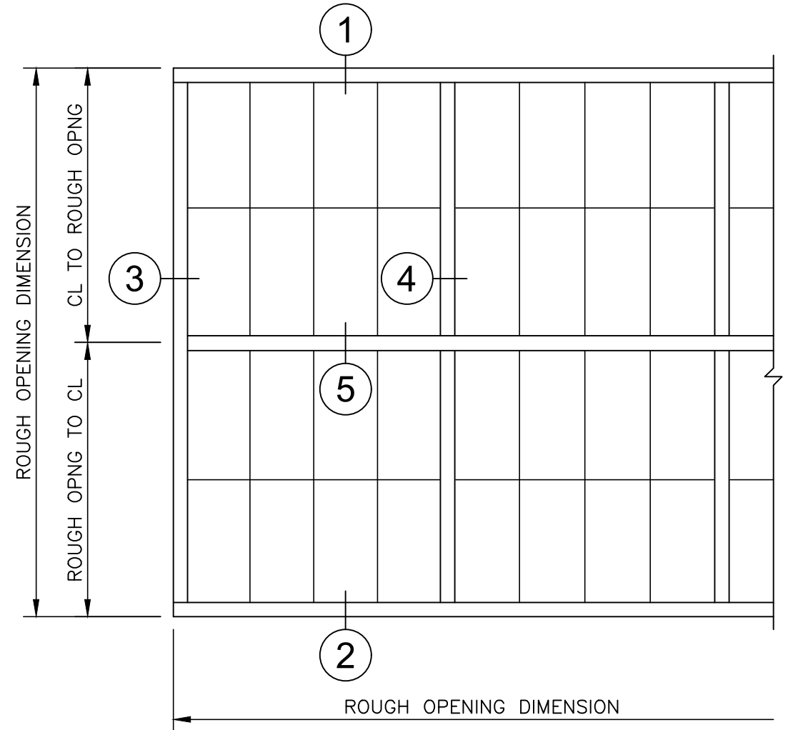
WALL ELEVATION
