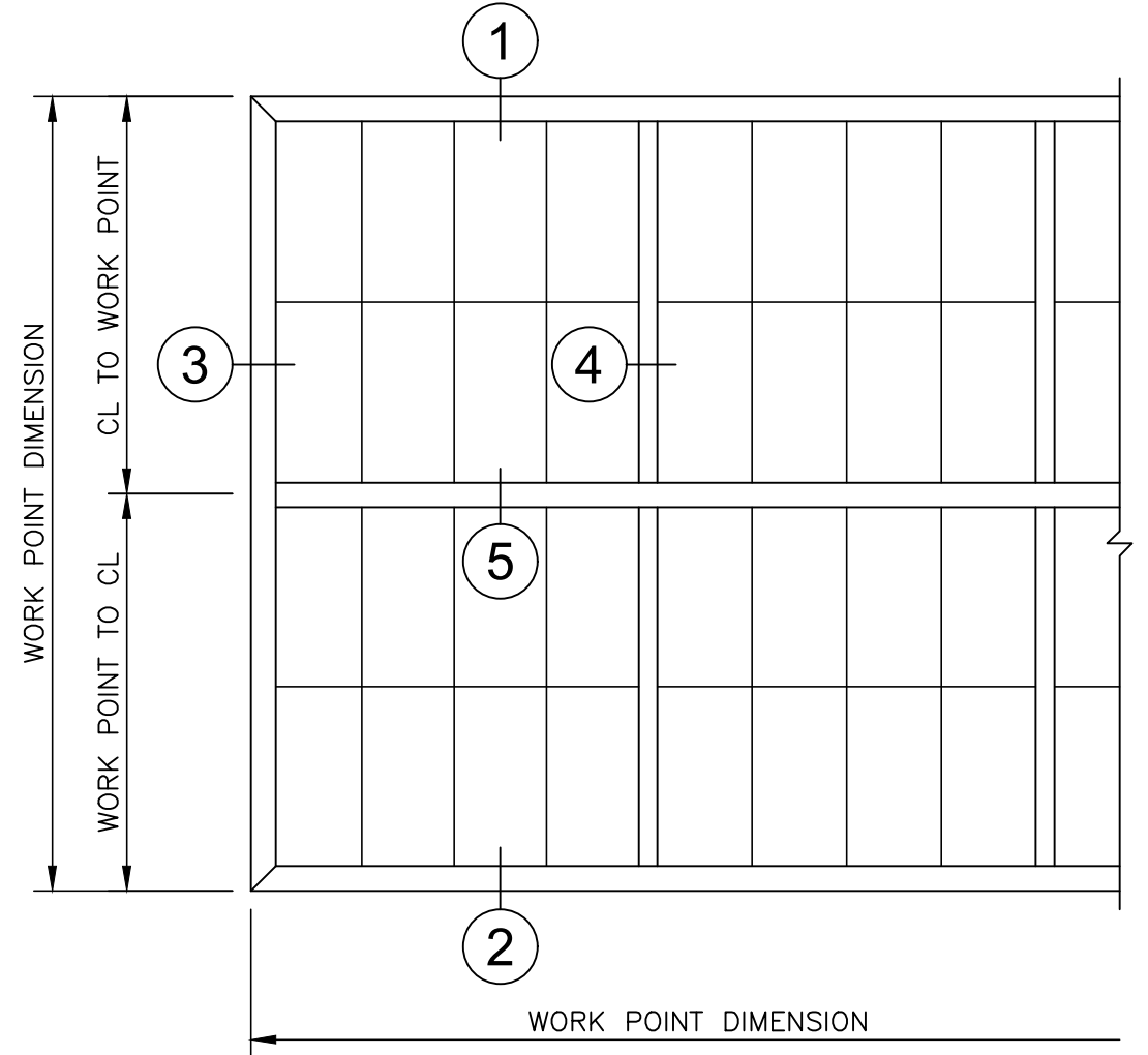
WALL ELEVATION
