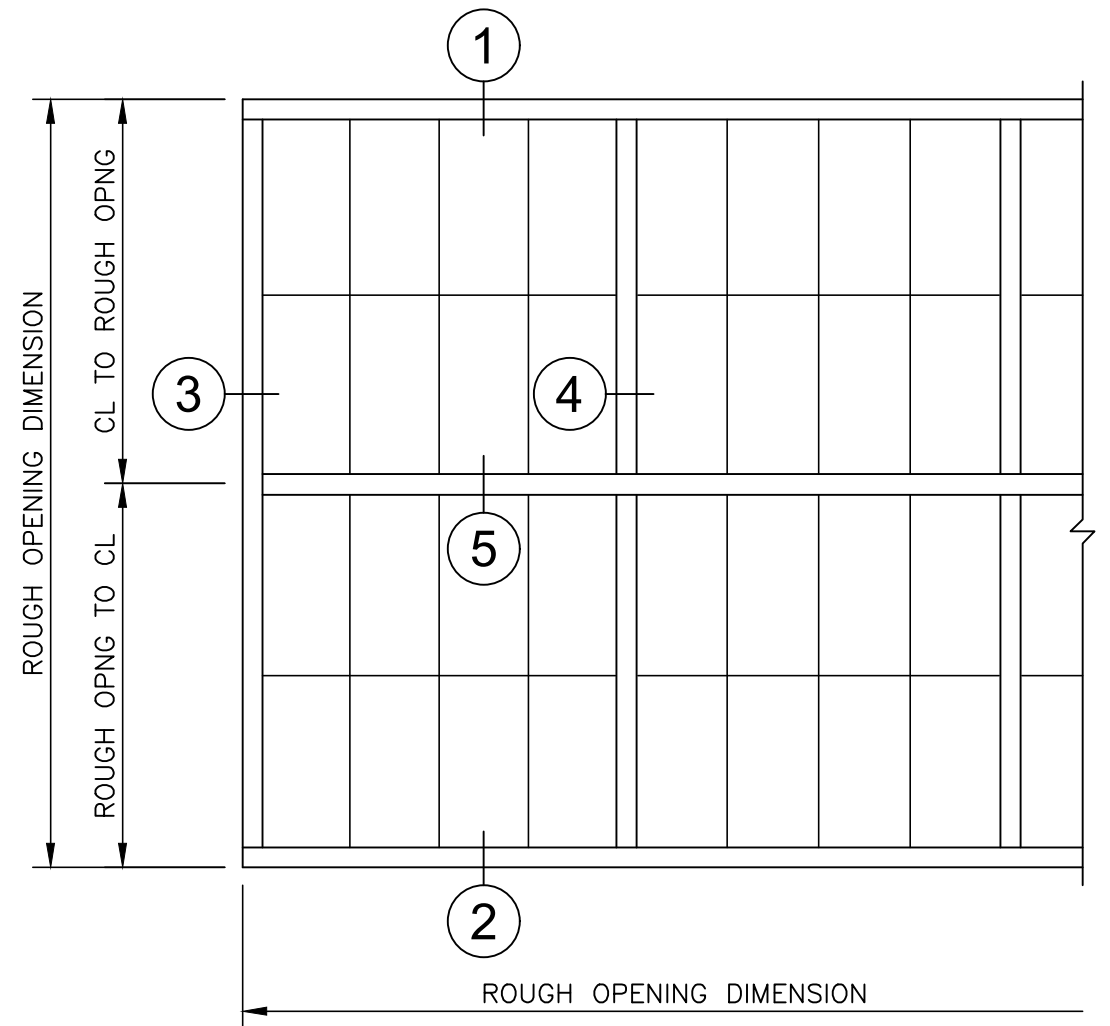
WALL ELEVATION
