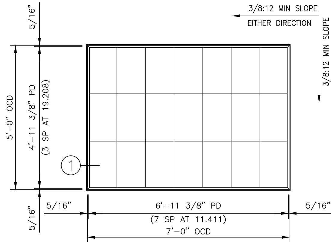
5' x 7' SKYLIGHT S-57-3A
