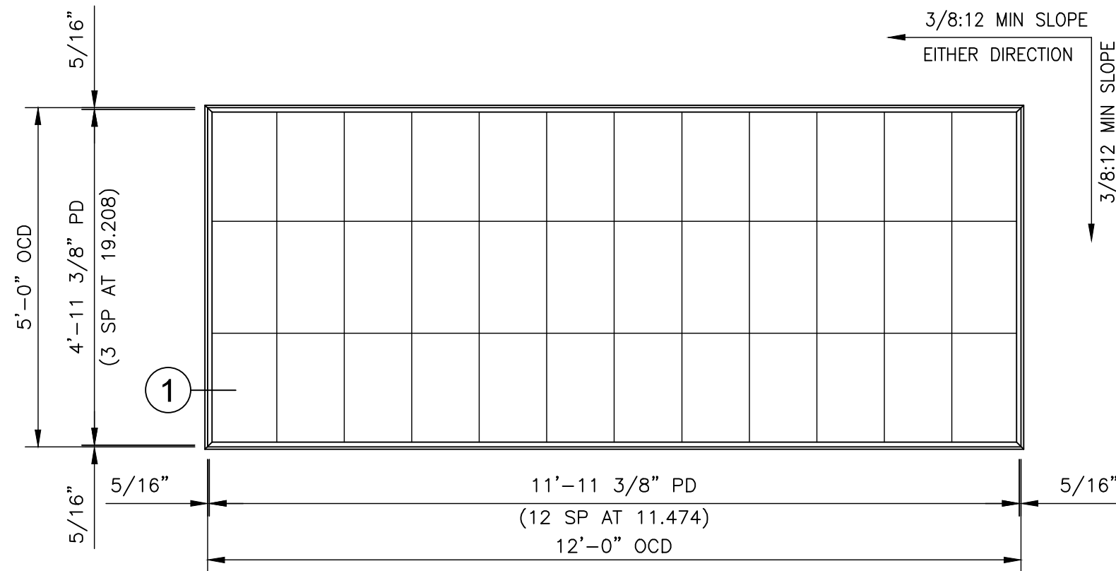
5' x 12' SKYLIGHT S-512-3A
