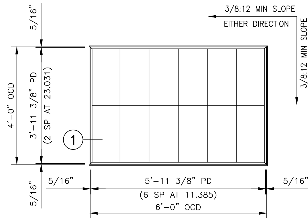
4' x 6' SKYLIGHT S-46-3A
