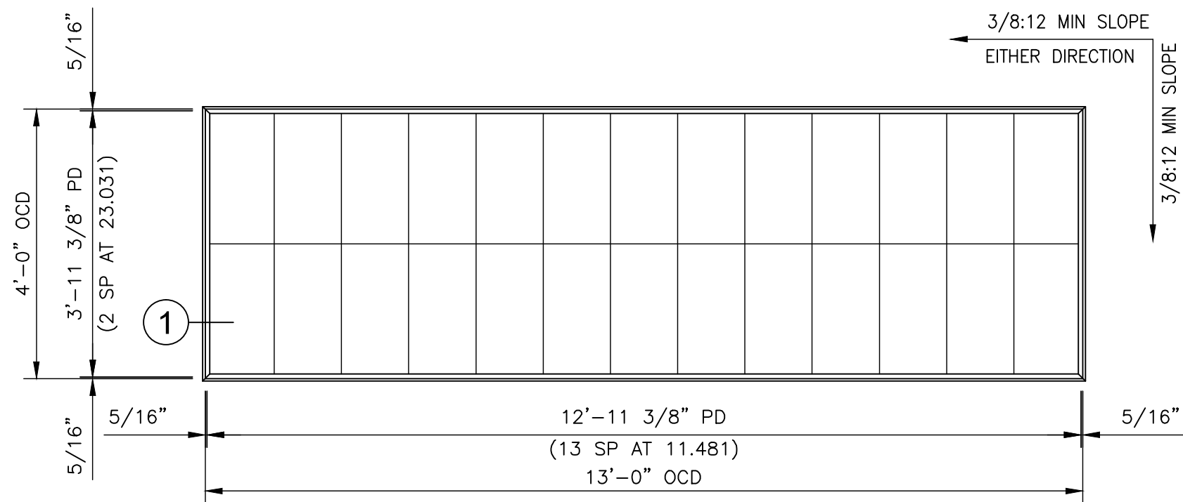
4' x 13' SKYLIGHT S-413-3A
