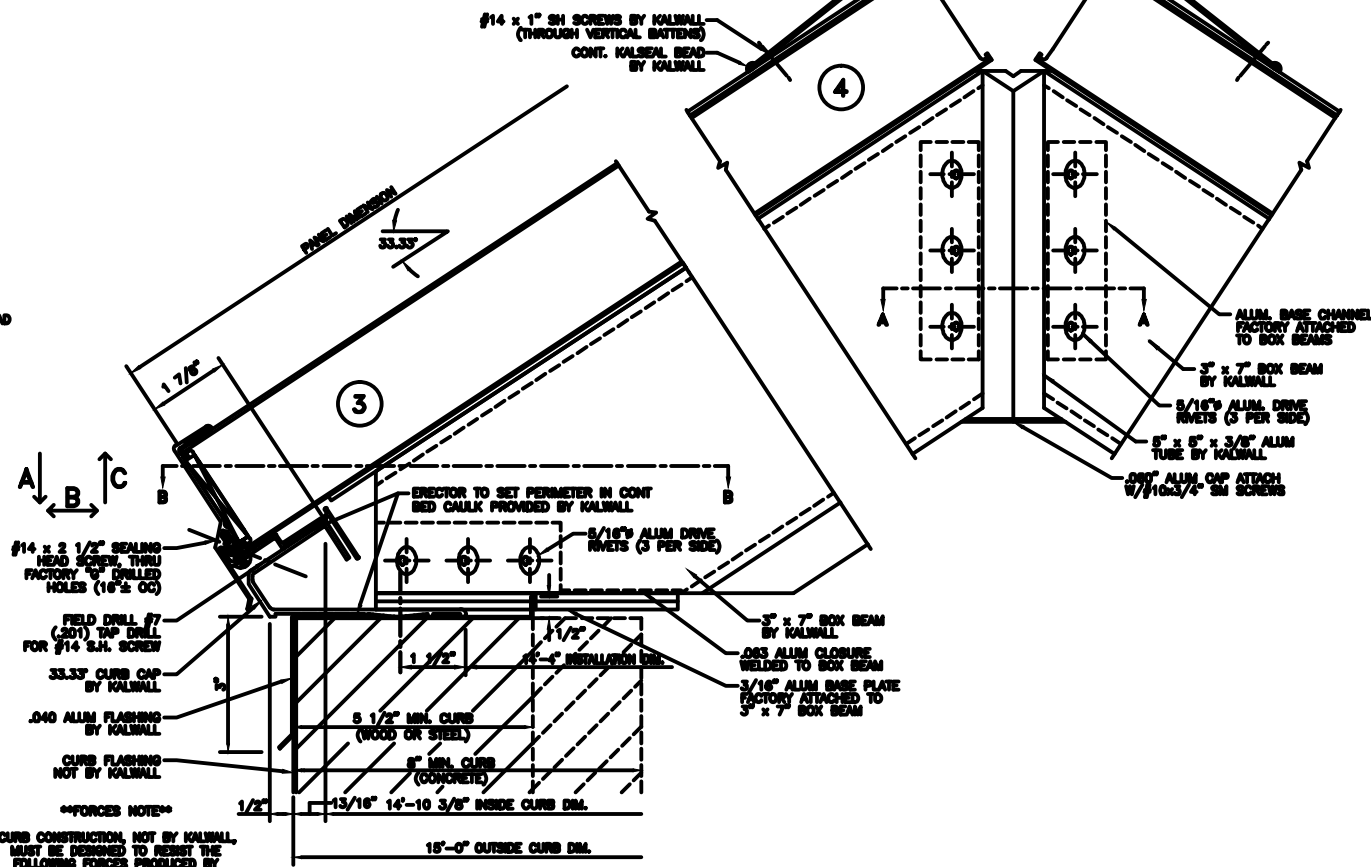
SECTION B-B
