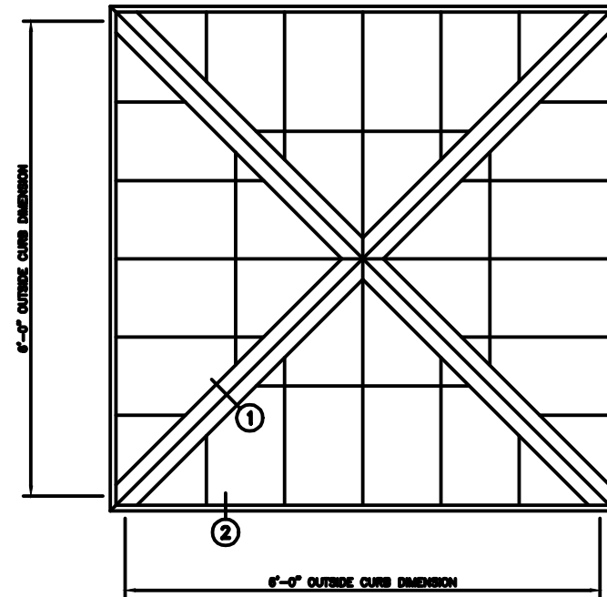
PYRAMID PLAN NOTE: SHIPPED IN 1 UNIT
