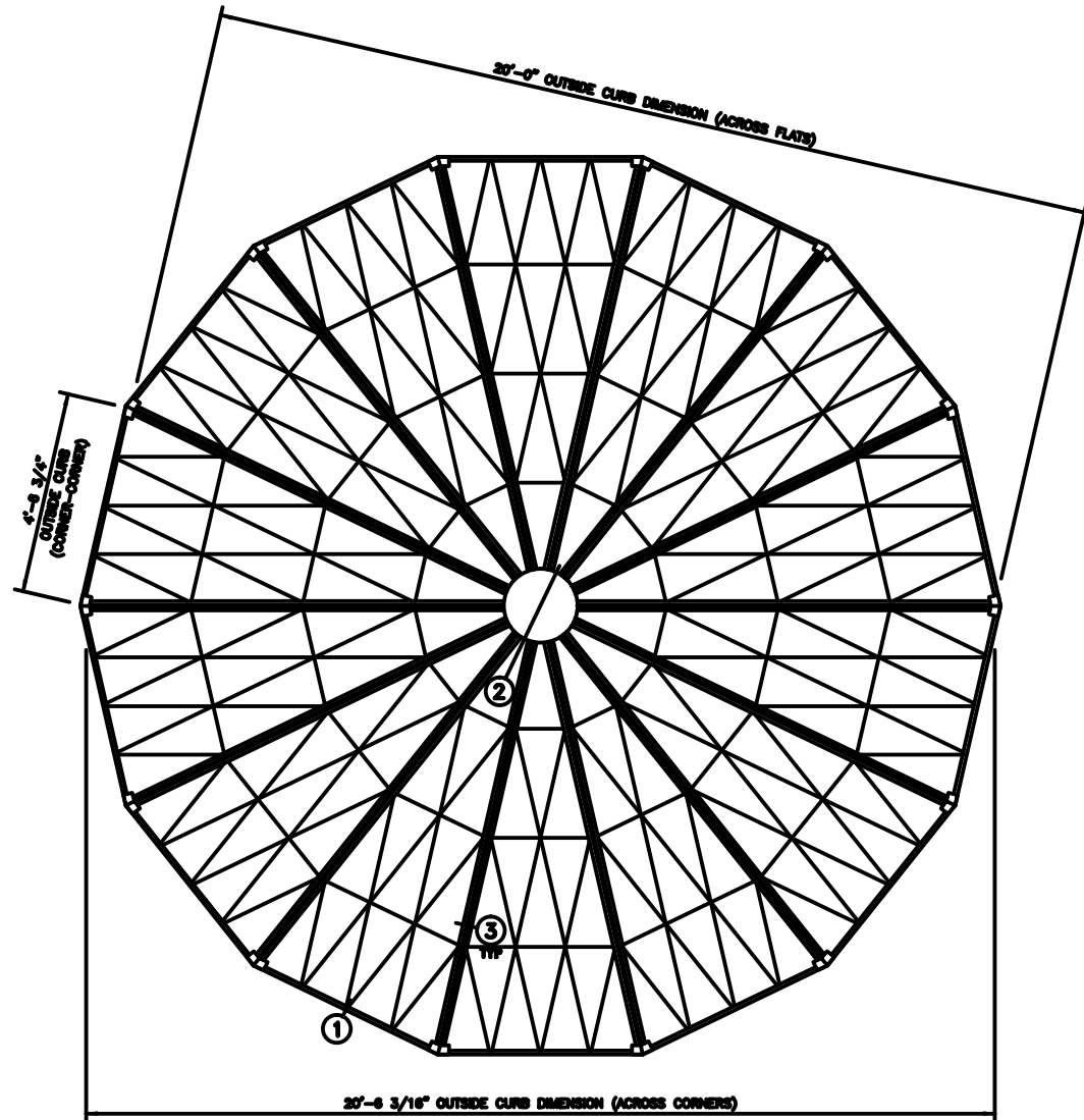
GEO ROOF PLAN NOTE: SHIPPED IN 14 UNITS
