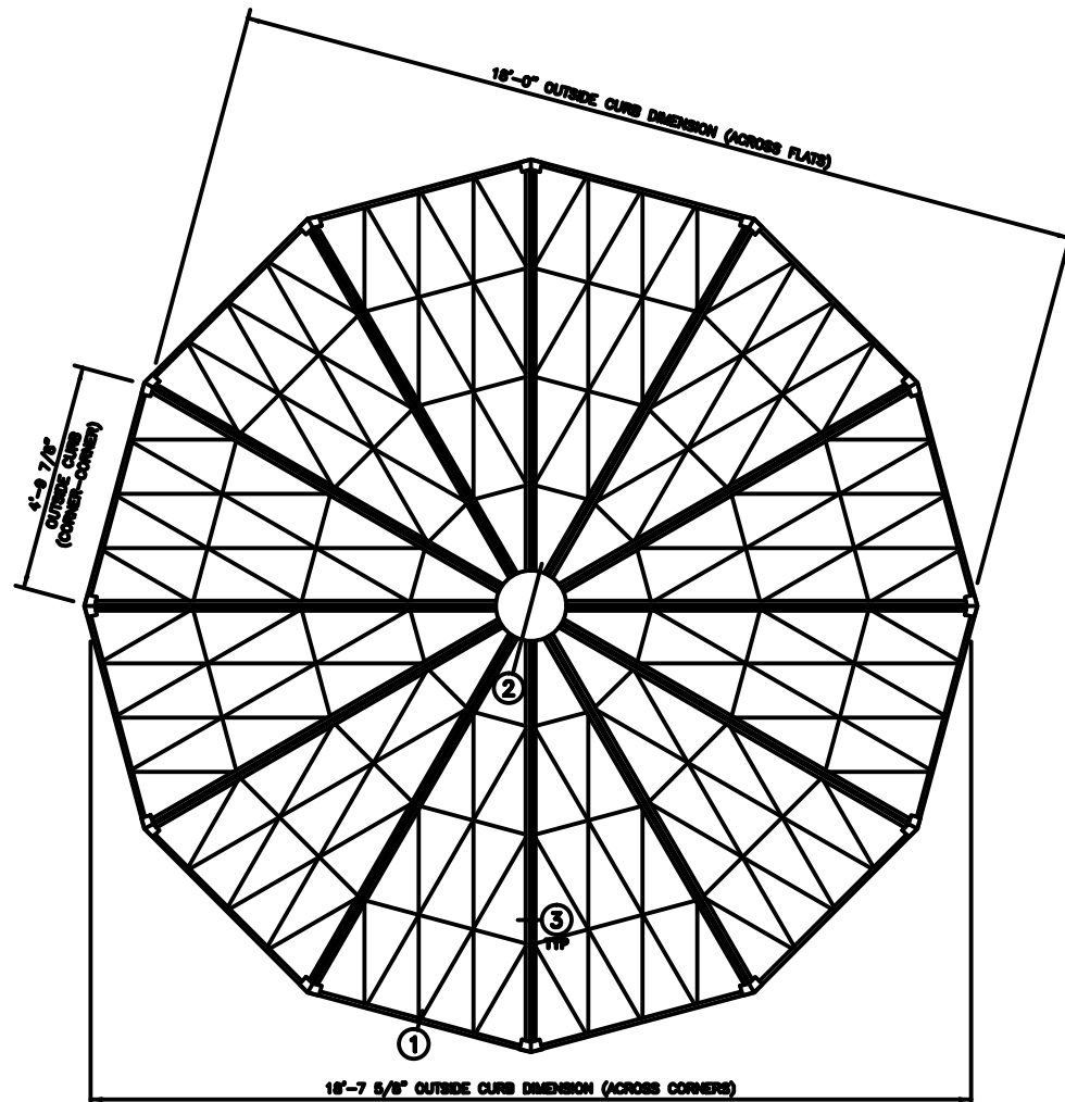
GEO ROOF PLAN NOTE: SHIPPED IN 12 UNITS
