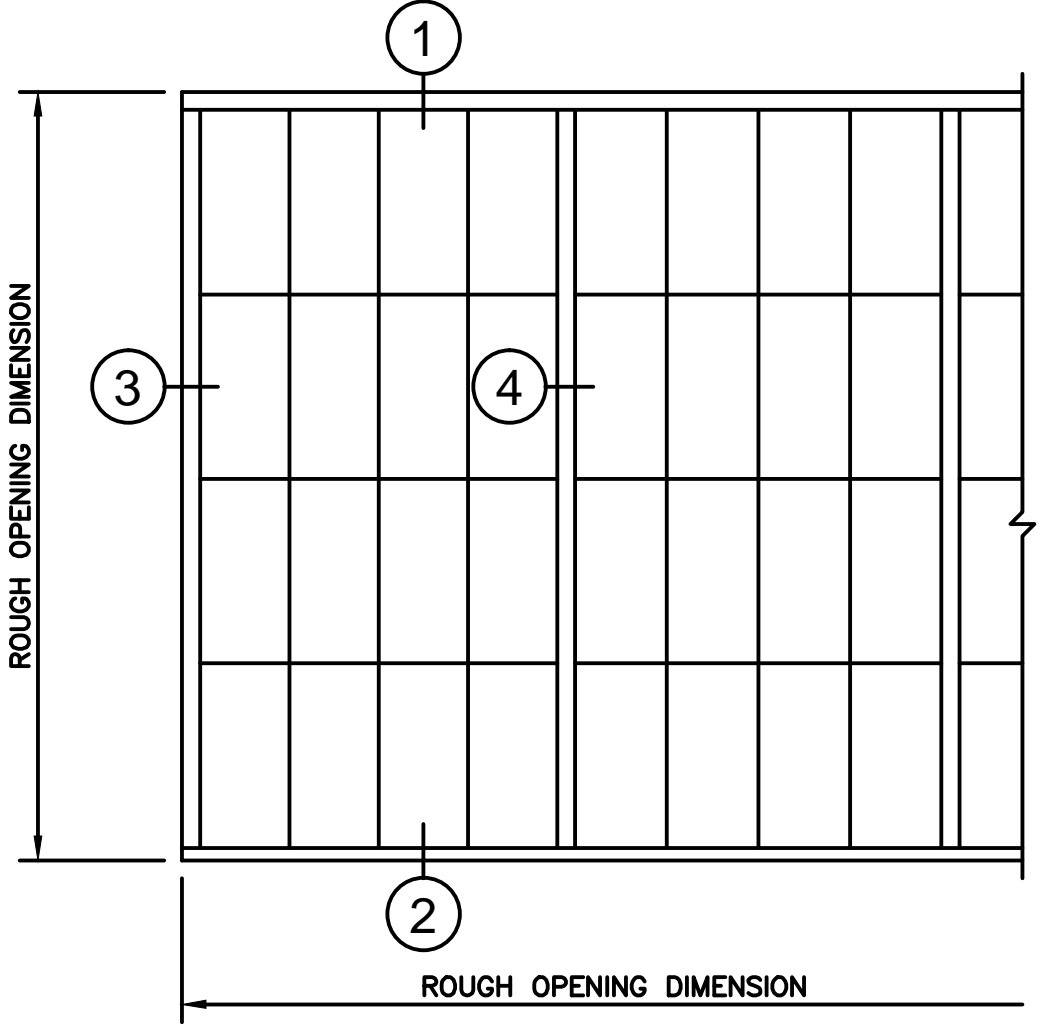
WALL ELEVATION
