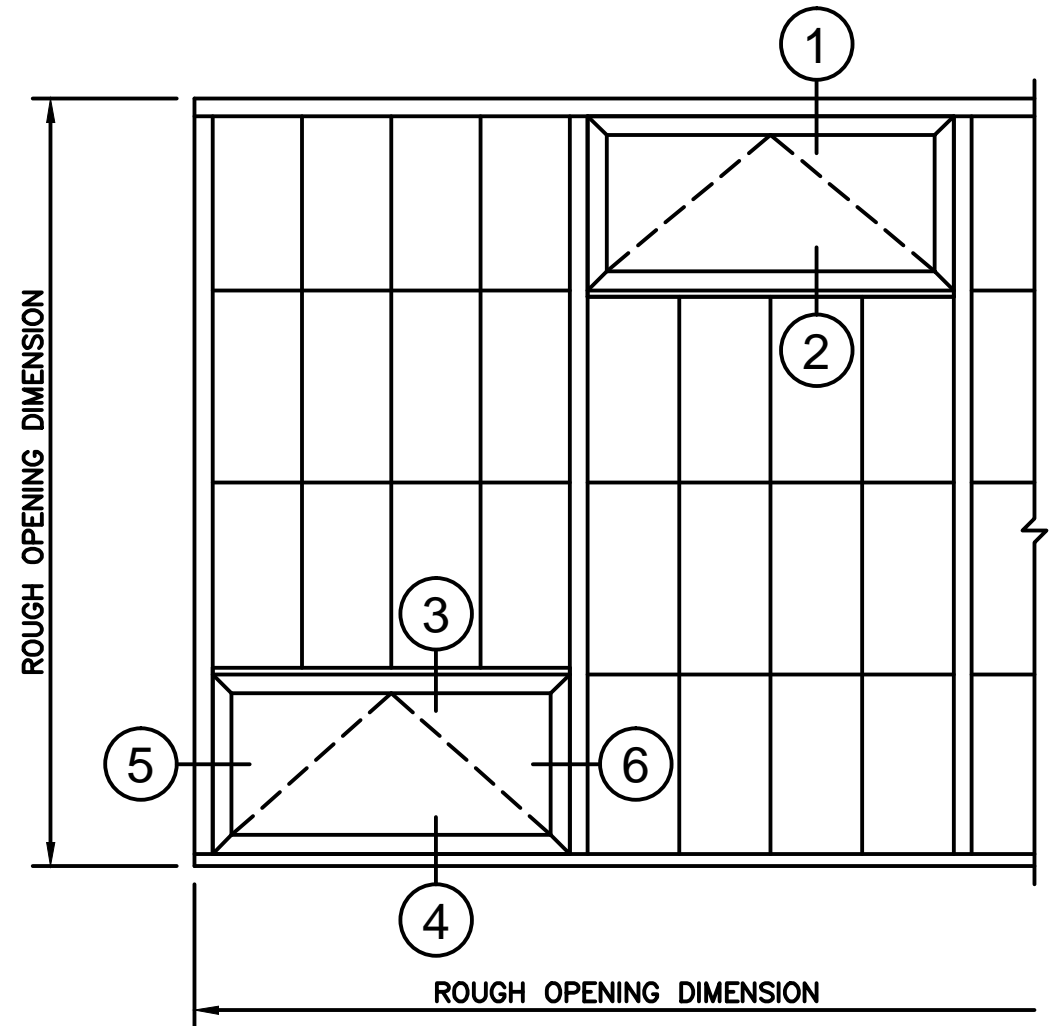
WALL ELEVATION
