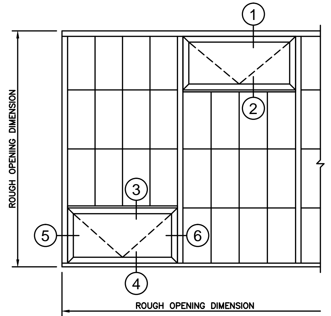
WALL ELEVATION
