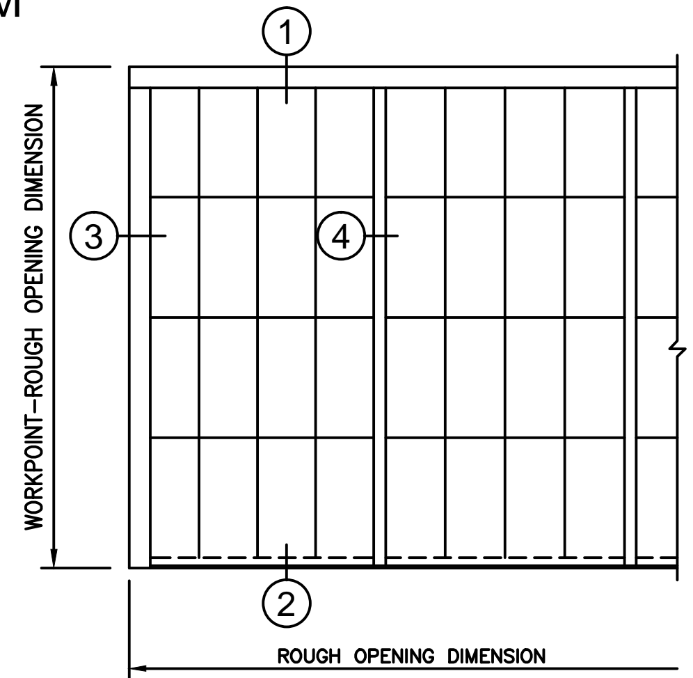
WALL ELEVATION
