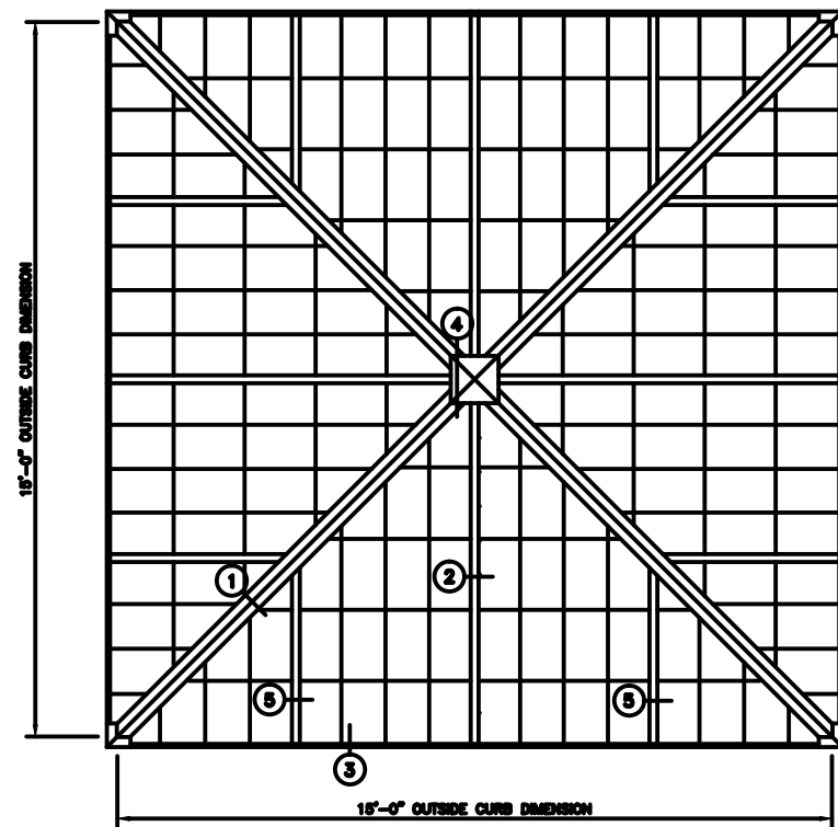
PYRAMID PLAN NOTE: SHIPPED IN 8 UNITS
