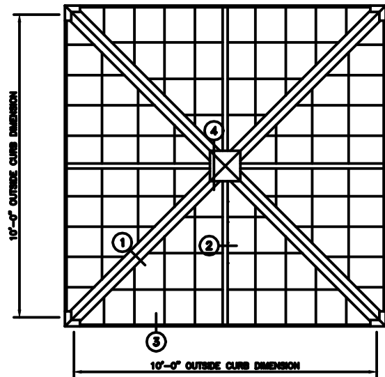
PYRAMID PLAN NOTE: SHIPPED IN 4 UNITS
