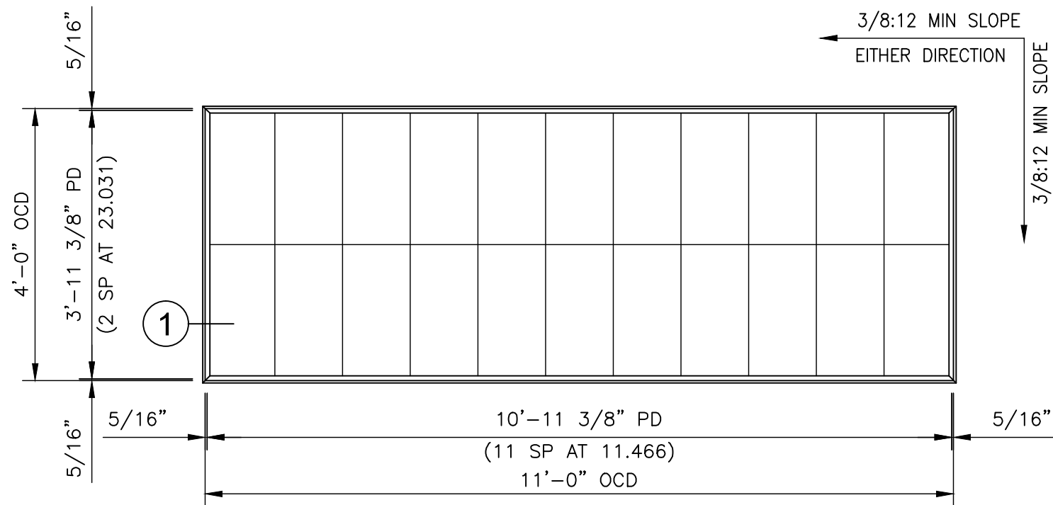
4' x 11' SKYLIGHT S-411-3A
