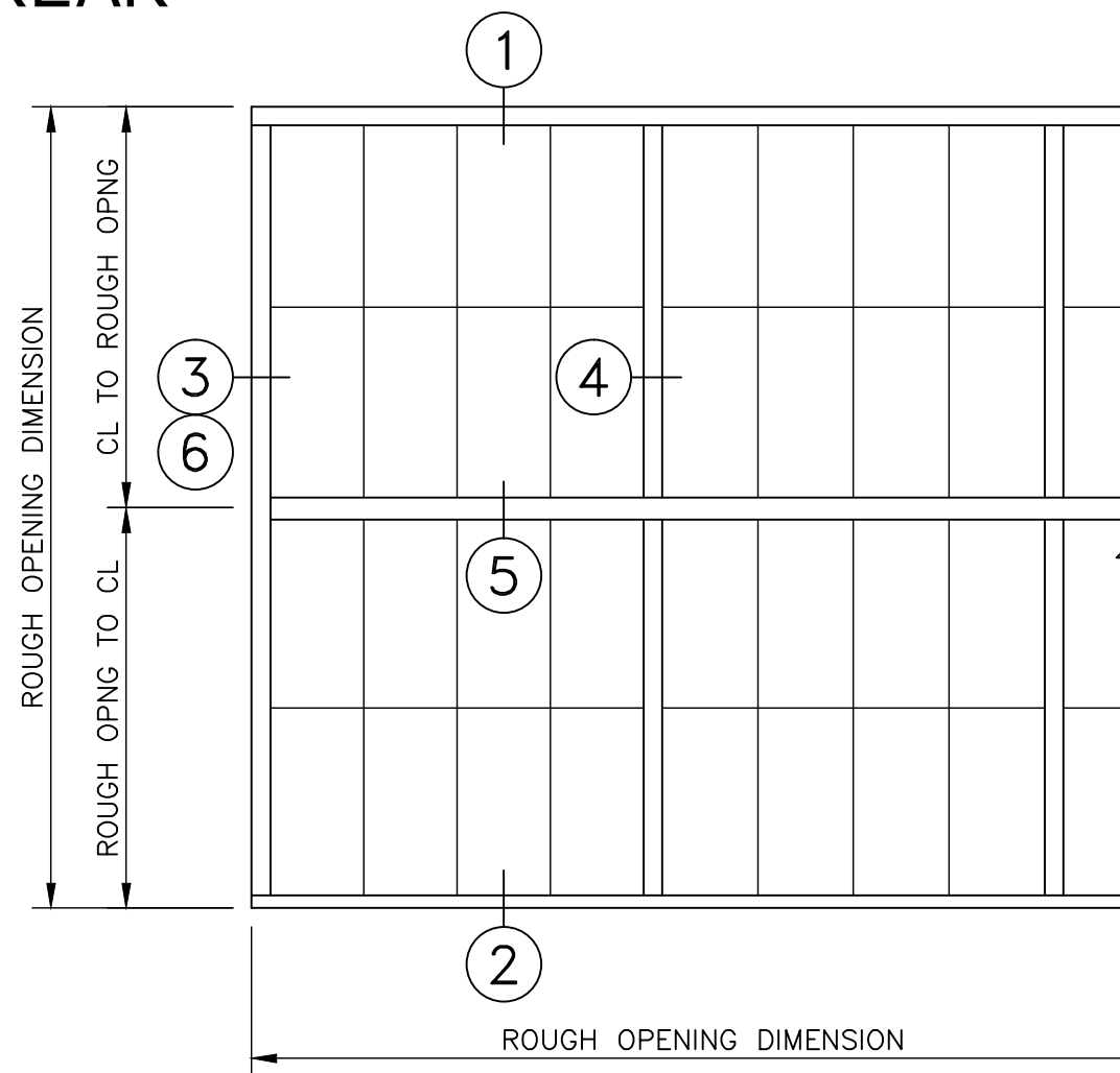
WALL ELEVATION
