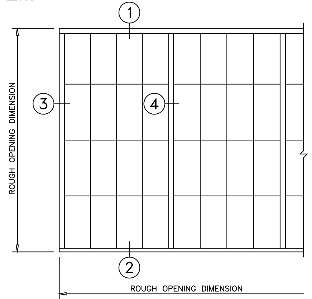
WALL ELEVATION
